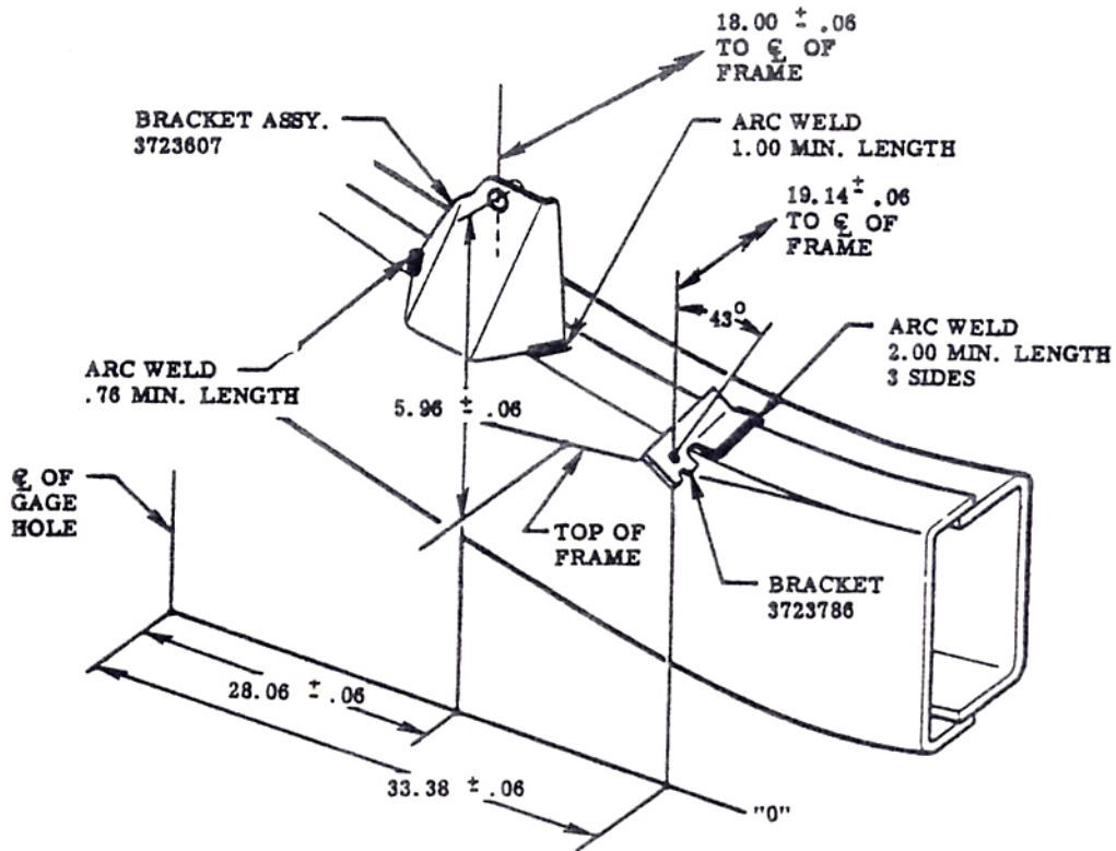
VIEW A
